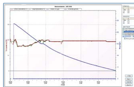
Pre-plotted and recorded fermentation curves for perfect temperature control and documentation
