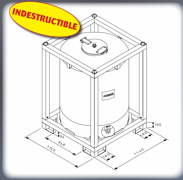
Paletank – stackable to 5 pieces and transportable on all types of transpallets and fork lifts
